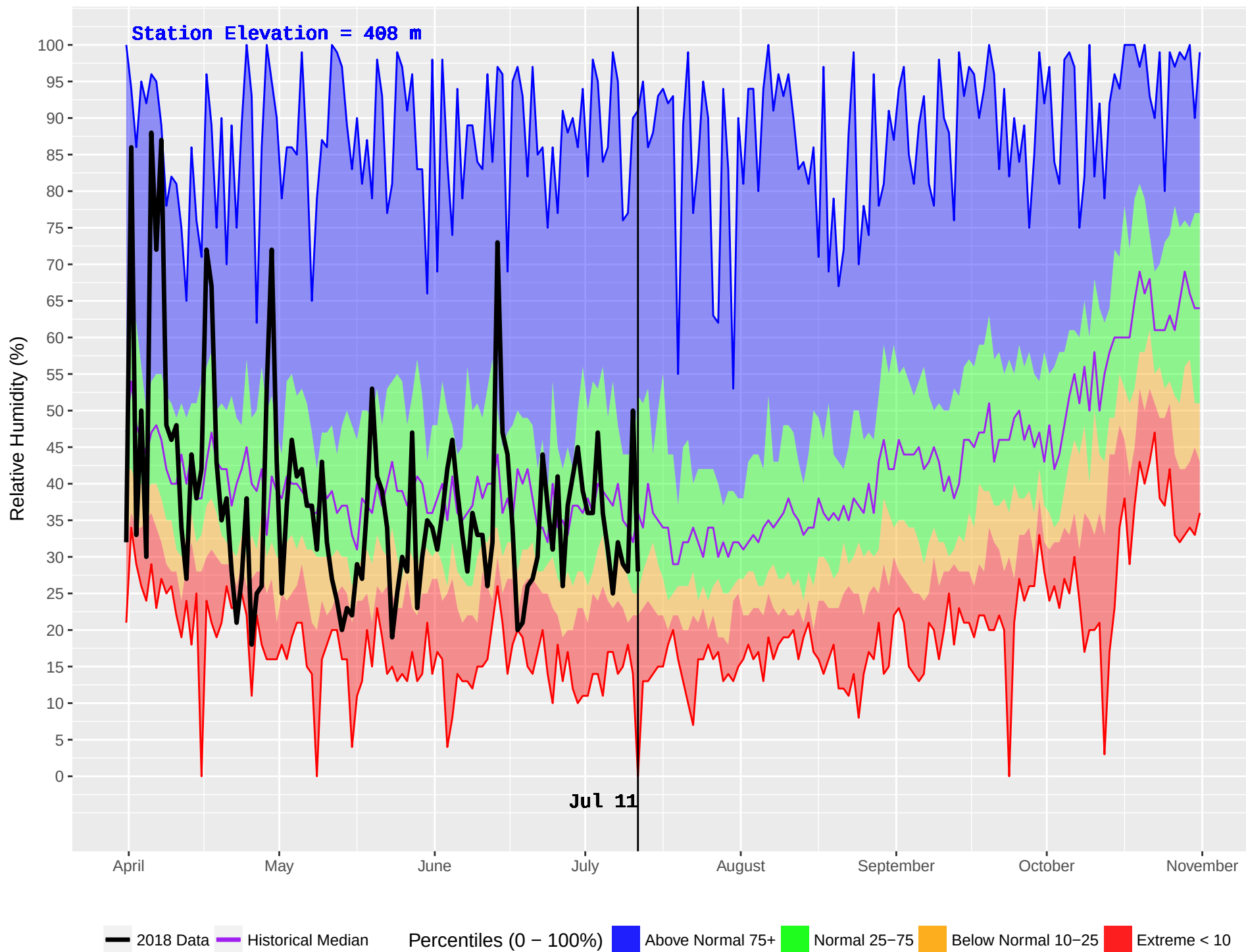
LILLOOET (280) : Historical (1977–2016) and Current (2018) Noon Relative Humidity
